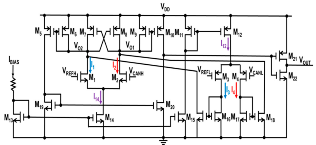
Figure 11. Schematic of hysteretic dual-to-single receiver.
