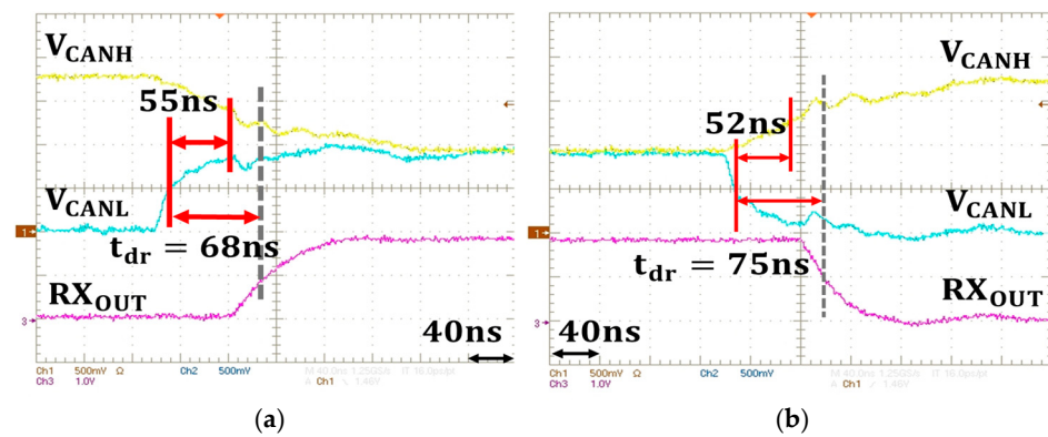
Figure 17. Timing errors with phase mismatch between V_{CANH} and V_{CANL} (a) t_{dr} , (b) t_{df} .
