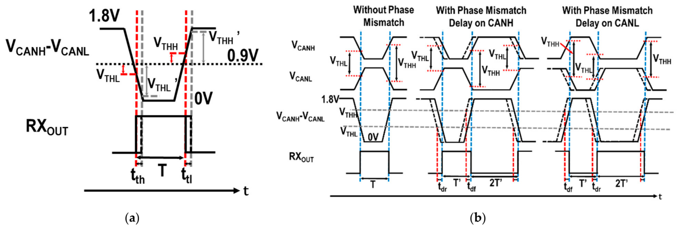
Figure 12. (a) RX_{OUT} 's pulse width relationship with V_{THH} and V_{THL} ; (b) Phase mismatch compensation under different situations.
