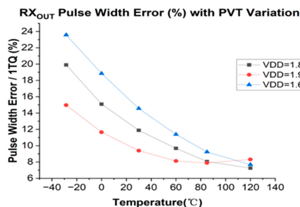
Figure 16. RX OUT pulse width error with temperature ( -28.5\text{ }^{\circ}\text{C} to 120\text{ }^{\circ}\text{C} ) and voltage ( V_{DD} = 1.8\text{ V}/1.98\text{ V}/1.62\text{ V} ) variation.
